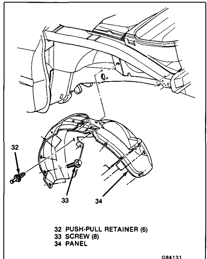
Fig. 14-Installing Rear Wheelhouse Panel
