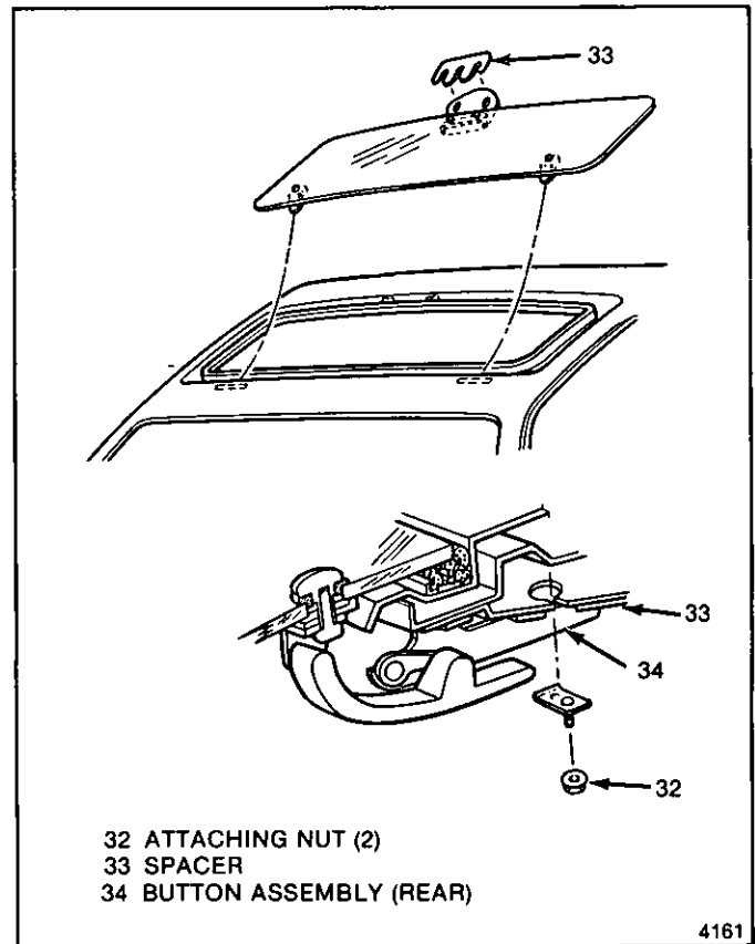
Fig. 8-11-Latch Adjustment
