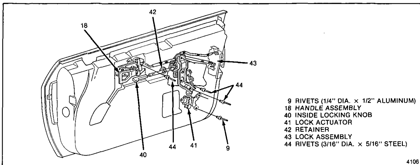
Fig. 5-11-Connecting Rods and Locking Rods
